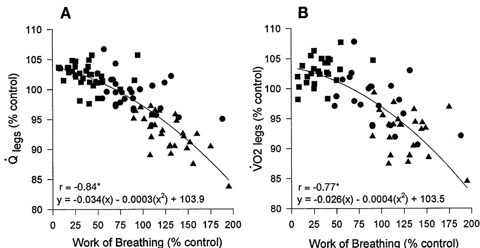
Fig. 3. Relative effects of changing Wb on \dot{Q}_{legs} and \dot{V}_{O_{2legs}} for all subjects using all trials. Percent control is calculated from 1st test from each testing session. A: \dot{Q}_{legs} is significantly related to Wb at \dot{V}_{O_{2max}} . B: \dot{V}_{O_{2legs}} is significantly related to Wb at \dot{V}_{O_{2max}} . The second measurements of blood flow, blood pressure, and blood samples of each test (2:00–2:30 min) were used for interpretation of data. Circles, control; squares, inspiratory unload; triangles, inspiratory load. *Significantly different, P < 0.05 .
